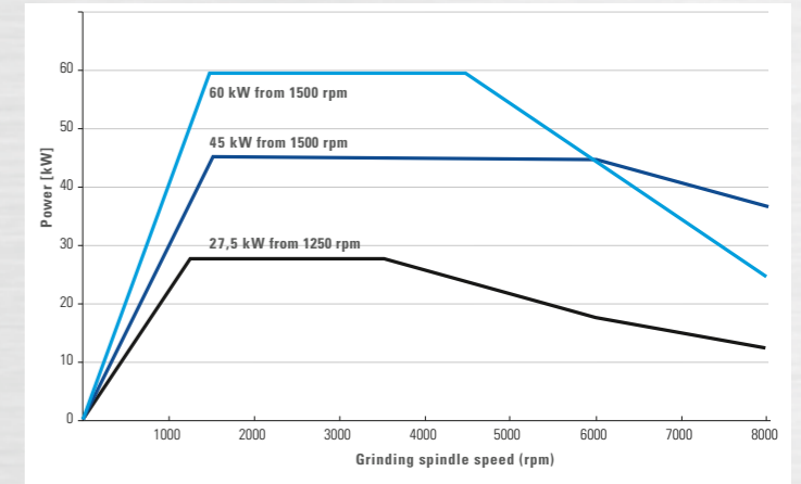
Grinding spindle drive power curves
