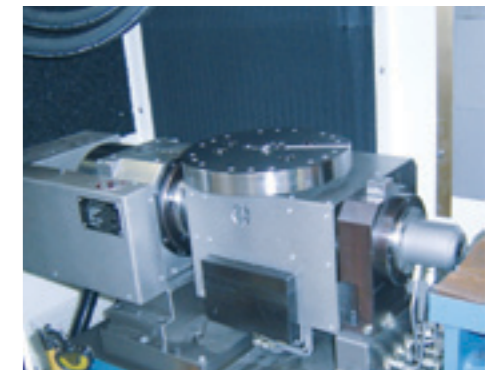
NC-indexing table , 1 or 2 axes, indexing accuracy +/- 1"
