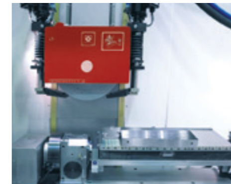
NC-tilting magnetic chuck , tilting range +/- 30° indexing accuracy +/- 1"
