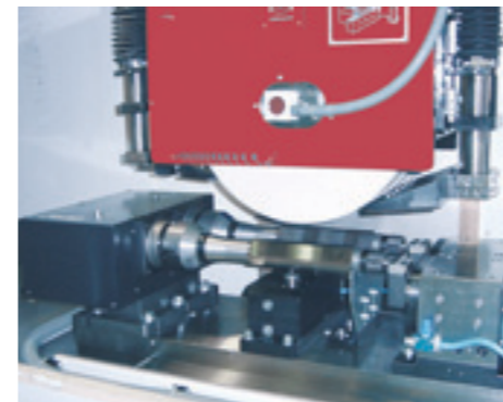
Twin-spindle NC-indexing table with tailstock , indexing accuracy +/- 3"
