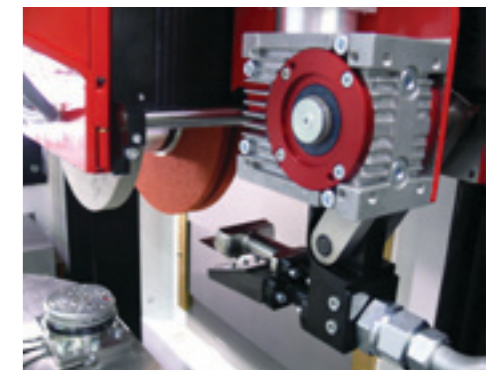
New way of grinding wheel cleaning, with newly developed nozzle positioner, 30% less grinding wheel wear, 30-40 bar nozzle pressure
