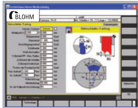
5-axes continuous path controlled grinding
