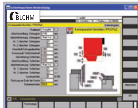
Contour parallel dressing
